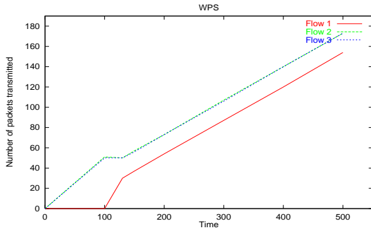
Figure 5.3 Service degradation: WPS (Credit bound = 30)
