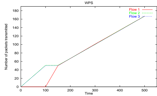
Figure 5.2 Service degradation: WPS (Credit bound = 50)
