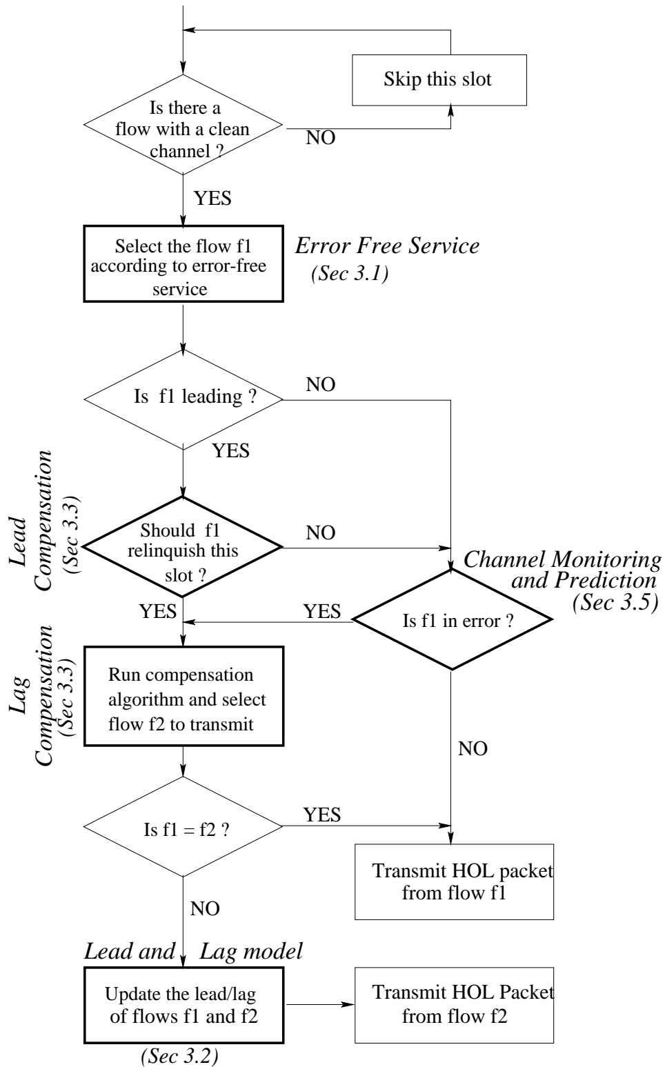
Figure 3.1 Interaction among the components of the unified wireless fair queuing architecture. The bold boxes indicate programmable components. In the lag compensation box, the alternate flow f_2 is constrained to be a backlogged flow that perceives a clean channel.
