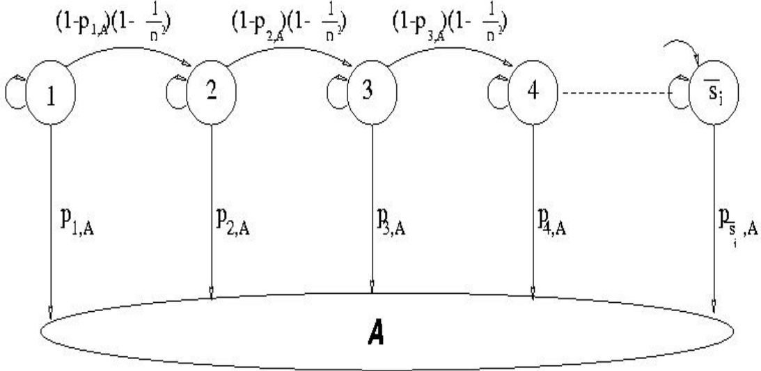
Fig. 5. The first time to reach the state \mathcal{A} in the Markov Chain gives an upper bound (in a stochastic order sense) on the time spent by a node while the dimension is i . The values of p_{s_i,A} are given by (4)-(6) in Lemma 4.2, and given by (11)-(13) in Lemma 5.3.
