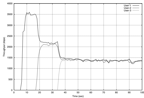
Fig. 7. QoS experiment: scenario 1.
