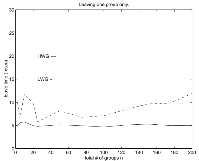
Figure 9. Leave one group
