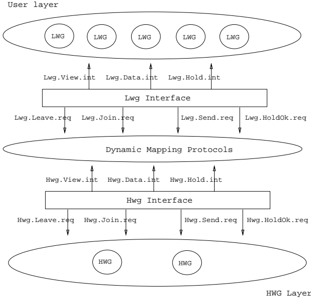
Figure 1. Light-Weight Group service interface
