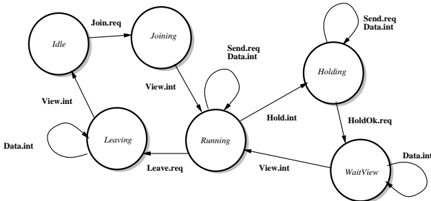
Figure 2. VS interface state machine
