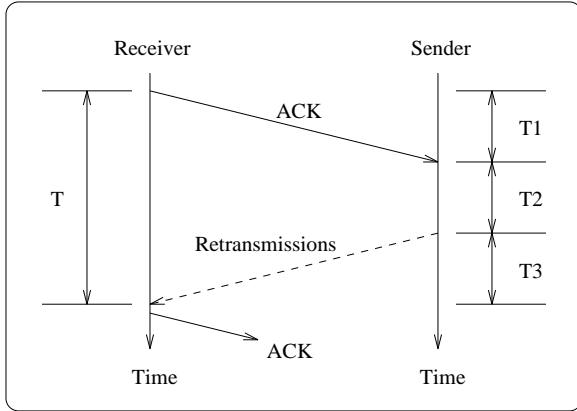
Figure 6: The components in calculating T_{ack}
