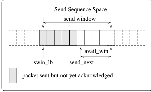
Figure 5: A sender's send window and related variables
